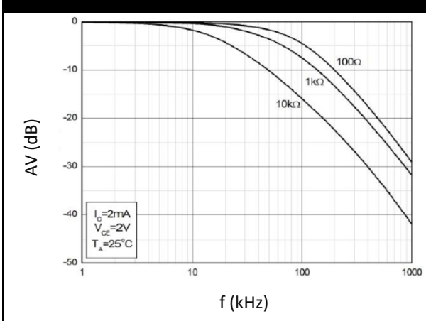
Frequency Response
