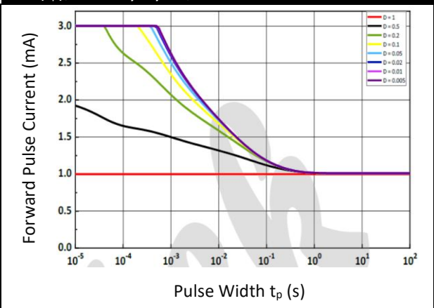
Permissible Pulse Handling Capability I_F = f(t_p) ; D = \text{Duty Cycle} ; T_s = 85^\circ\text{C}
