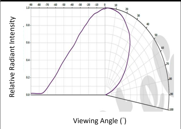
Directive Radiation (L=0)
